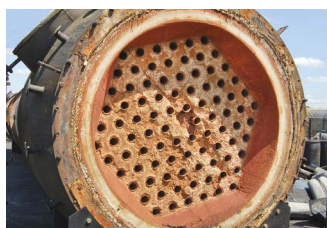
Opening of an air preheater with refractory lining
